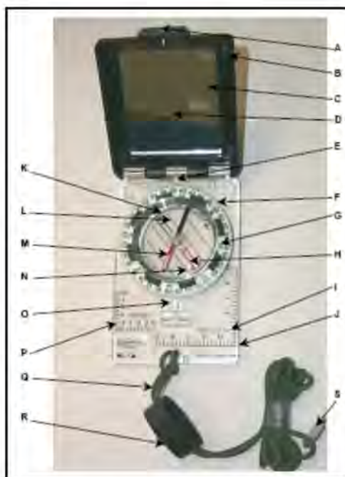
Figure 12-3-1 Boussole
